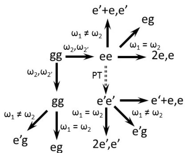
Figure 11.12: Liouville pathways for ???. gg and ee designate ground- and excited-state populations, the eg , 2e,e , and e'+e,e represent the excitonic and biexcitonic output coherences, and the arrows are labeled with the frequencies or population transfer responsible for the transitions. e and e' represent either A or B excitonic states.
