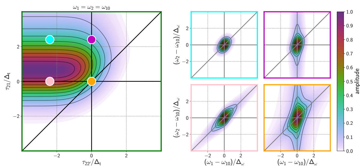
Figure 9.6: Changes to the 2D frequency response of a single Liouville pathway ( I_\gamma ) at different delay values. The normalized dephasing rate is \Gamma_{10}\Delta_t = 1 . Left: The 2D delay response of pathway I_\gamma at triple resonance. Right: The 2D frequency response of pathway I_\gamma at different delay values. The delays at which the 2D frequency plots are collected are indicated on the delay plot; compare 2D spectrum frame color with dot color on 2D delay plot.
