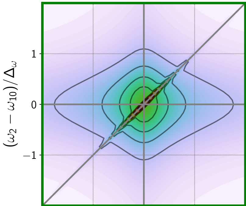
Steady State, \Gamma_{11}\Delta_t \rightarrow 0
