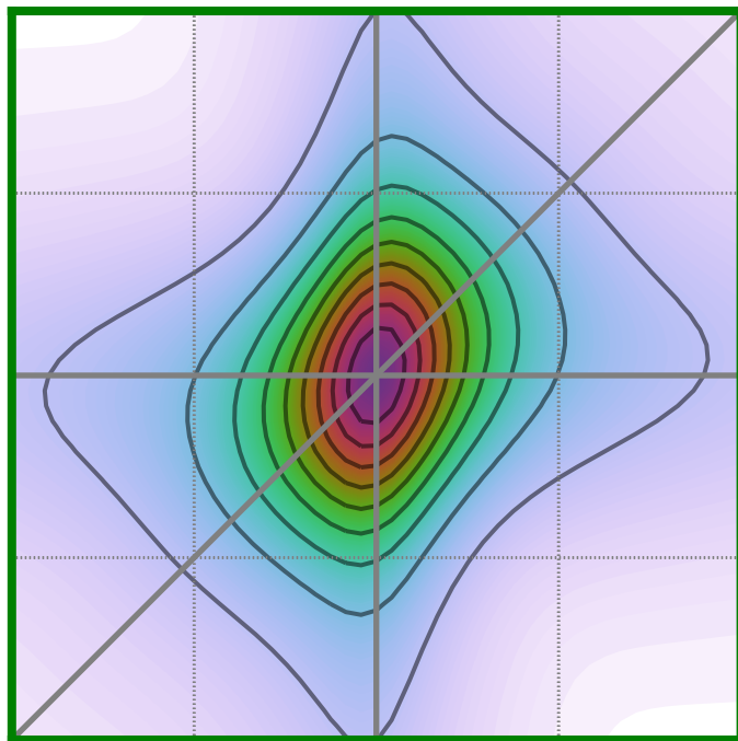
Steady State, \Gamma_{11}\Delta_t = 1
