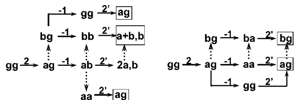
FIGURE 9. Representative coherence transfer pathways for two different phase matching conditions. The dotted arrows represent coherence transfer transitions. The emitting coherences are in boxes.
