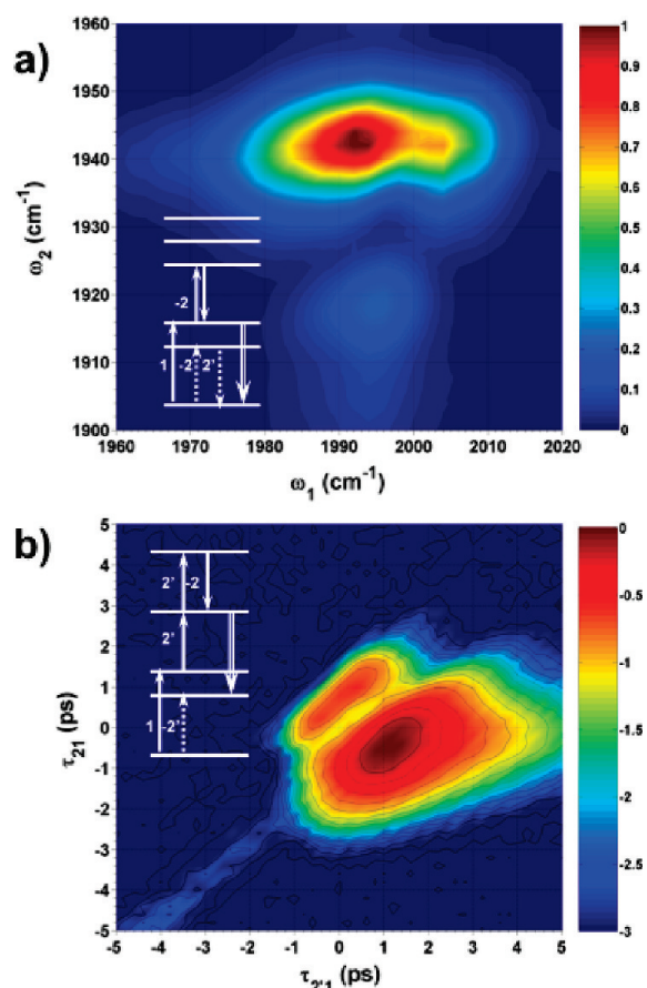
FIGURE 11. Changes when the excitation intensity is raised and higher order processes become important. (a) TRIVE FWM 2D spectrum scanning \omega_1 and \omega_2 near the \text{Ni}(\text{CO})_2 with \omega_m = 2002 \text{ cm}^{-1} and (\tau_{2'1}, \tau_{21}) = (2, 1) \text{ ps} (pathway IA). (b) \tau_{2'1} and \tau_{21} scan with (\omega_1, \omega_2, \omega_m) = (2002, 1931, 1982) \text{ cm}^{-1} .
