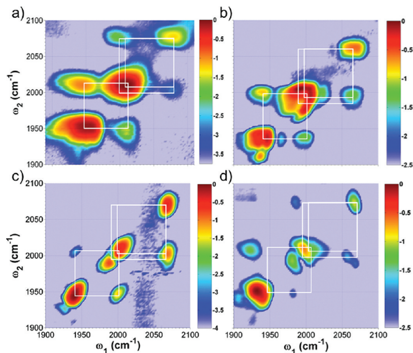
FIGURE 2. Representative TRIVE FWM 2D spectra of Ni(CO) 2 /Ni(CO) 3 scanning excitation frequencies with ( \tau_{21}, \tau_{21} ) values of (a) (0,0), (b) (2,1), (c) (2,1), and (d) (-1,2) ps. For panel a, there was no monochromator; for panels b, c, and d, \omega_m = \omega_1 . Boxes define vibrational energies of Ni(CO) 2 and Ni(CO) 3 (table 1).
