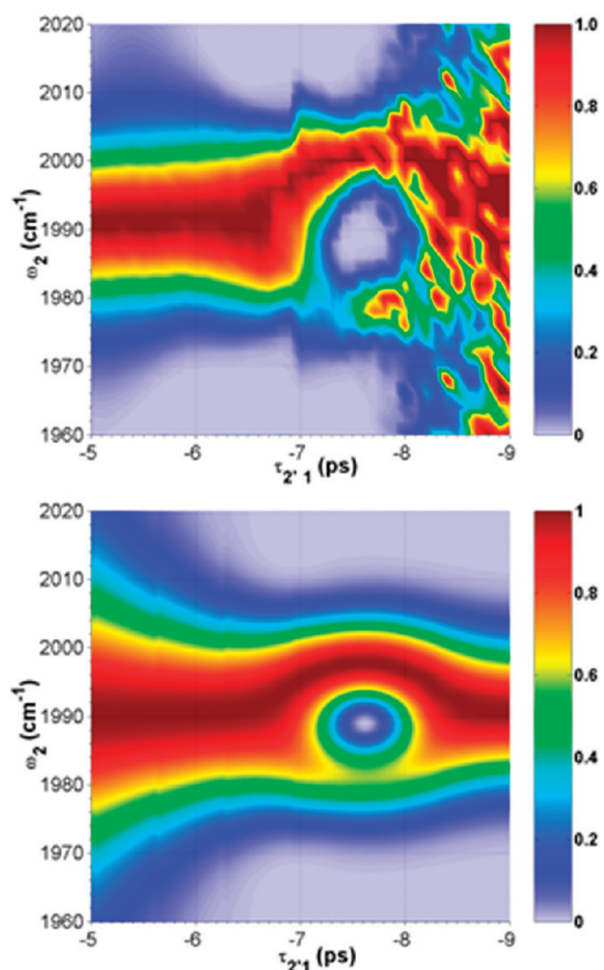
FIGURE 3. Experimental (top) and simulated (bottom) dependence of resonance when \omega_1 = 2069 \text{ cm}^{-1} , \tau_{21} = -5 \text{ ps} , and \omega_2 and \tau_{2,1} are scanned. Each vertical slice is normalized to most intense data point. 32 Reproduced with permission from ref 32. Copyright 2007 American Chemical Society.
