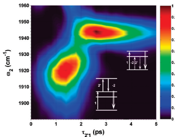
FIGURE 7. TRIVE FWM intensity dependence (linear) on \omega_2 and \tau_{2'1} when \omega_1 = \omega_m = 2002 \text{ cm}^{-1} and \tau_{21} = 2 \text{ ps} and example WMEI diagrams for pathways I and II.
