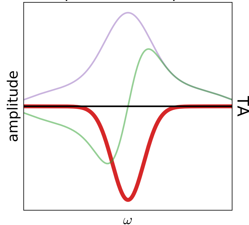
probe lineshape
